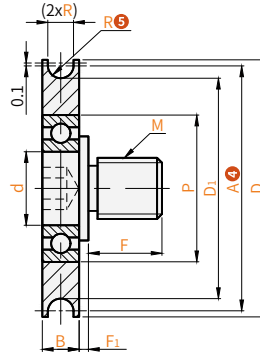
External thread type CFDJ-C2E1/C2N1/A1H1/S1W-Q
