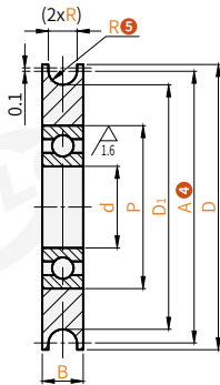
Standard type CFDJ-C2E1/C2N1/A1H1/S1W-P
