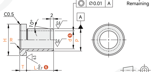
Thin-wall type FTDD-M2W/M2N1/S6W-B1D7/B1D8
