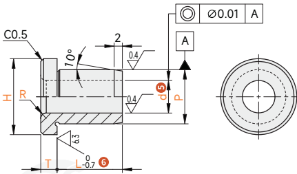
Standard type FTDD-M2W/M2N1/S6W-BD7/BD8
