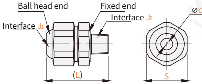
Internal and external thread type GSHL-K6
