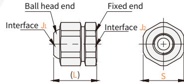
Internal thread type GSHL-K1
